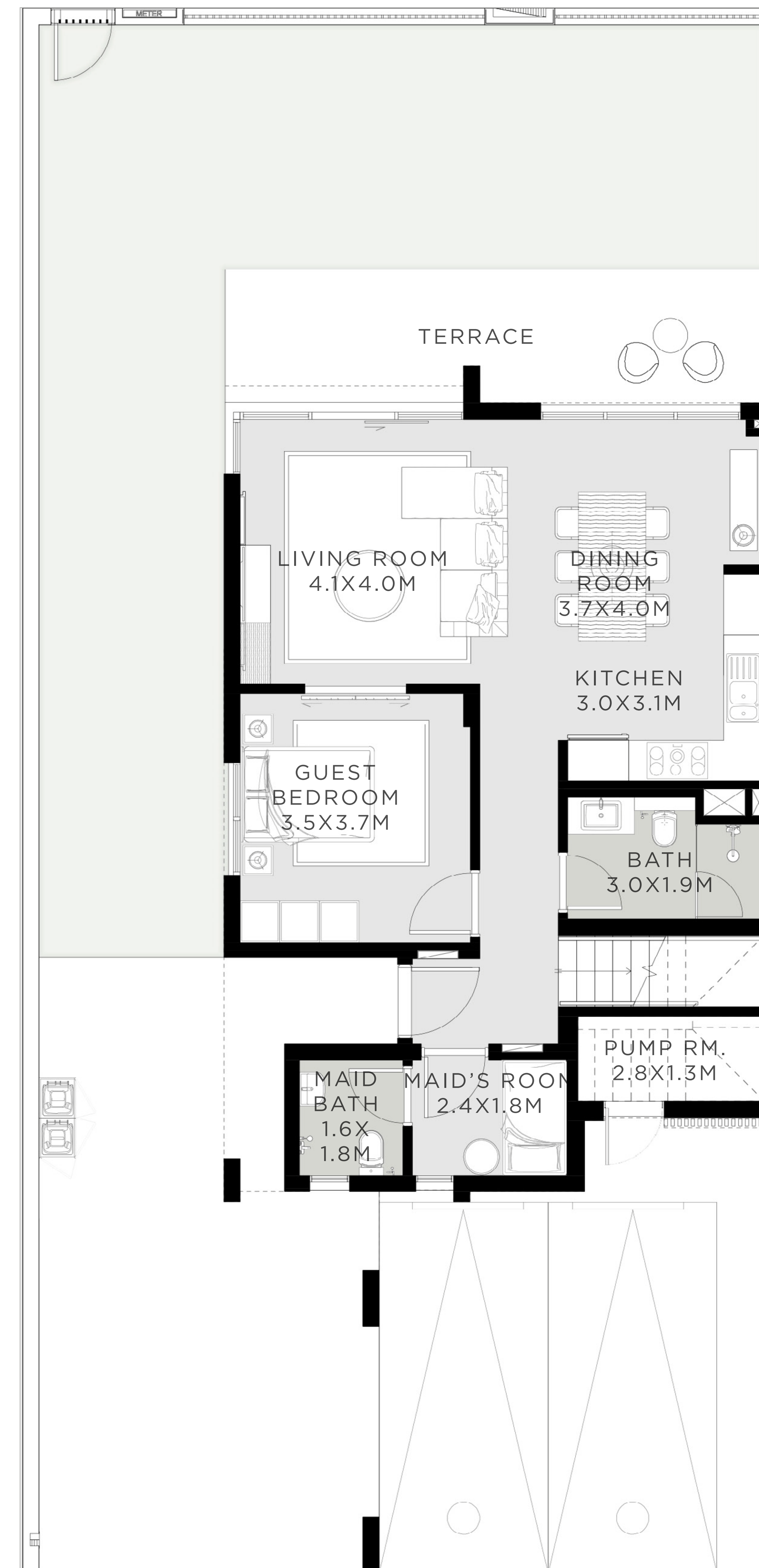
GROUND FLOOR
